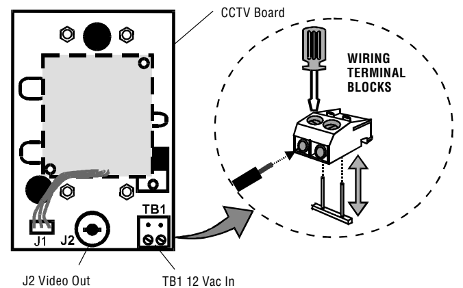
FIGURE 2: POWER AND VIDEO CONNECTIONS
