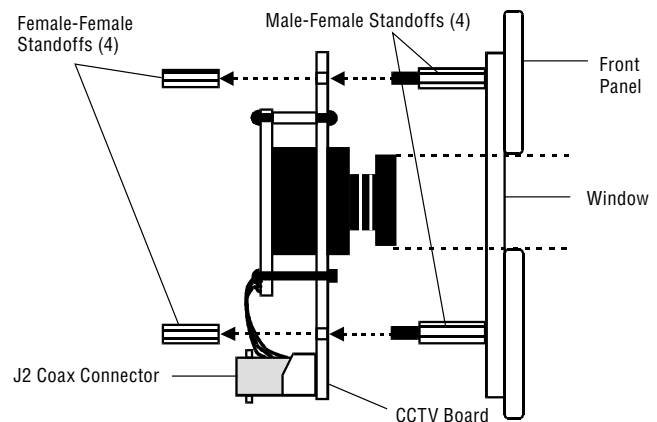
FIGURE 1: MOUNTING THE CCTV BOARD
